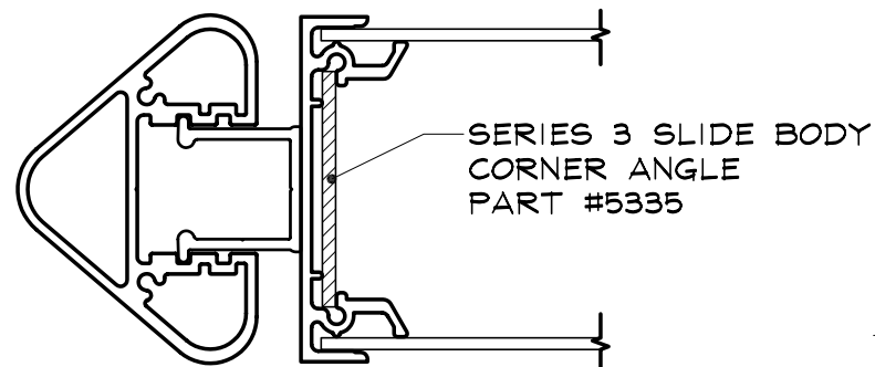
3/8" REVEAL POSITION
