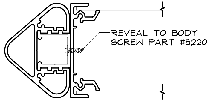
0" REVEAL POSITION
